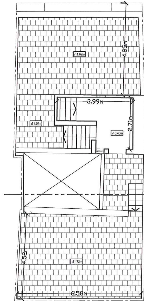
EXISTING ROOF LEVEL SCALE 1:100
