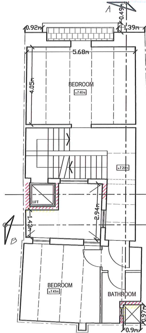
APPROVED/PROPOSED SECOND FLOOR SCALE 1:100
