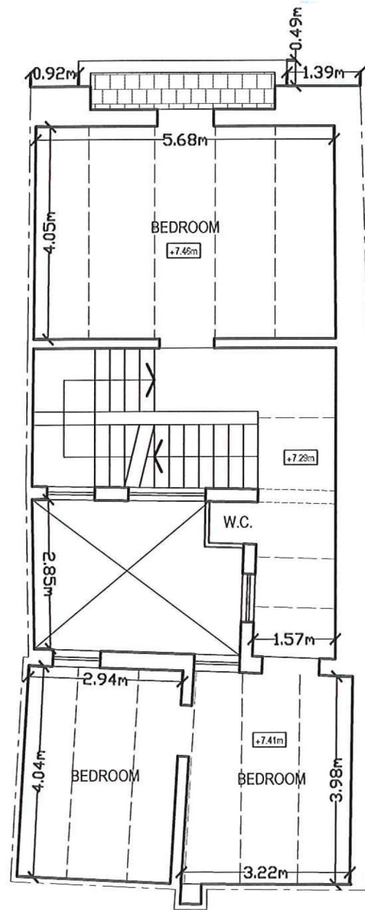
EXISTING SECOND FLOOR SCALE 1:100
