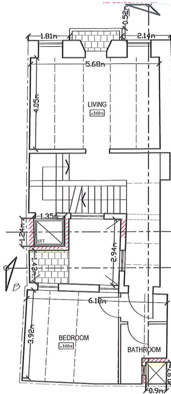
APPROVED/PROPOSED FIRST FLOOR SCALE 1:100
